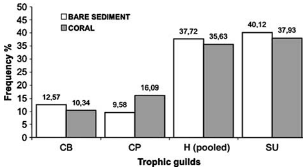
Fig. 5 Trophic guilds from mollusc assemblages in tanatocoenoses. CB browsing carnivores, CP predatory carnivorous, H (both microalgalivory and herbivores), SU suspension feeders
